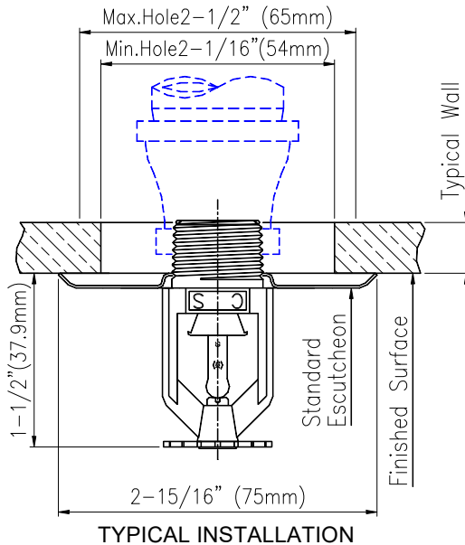
FIGURE C : MODEL NX025/NX026 PENDENT SPRINKLER INSTALLED WITH A STANDARD ESCUTCHEON
