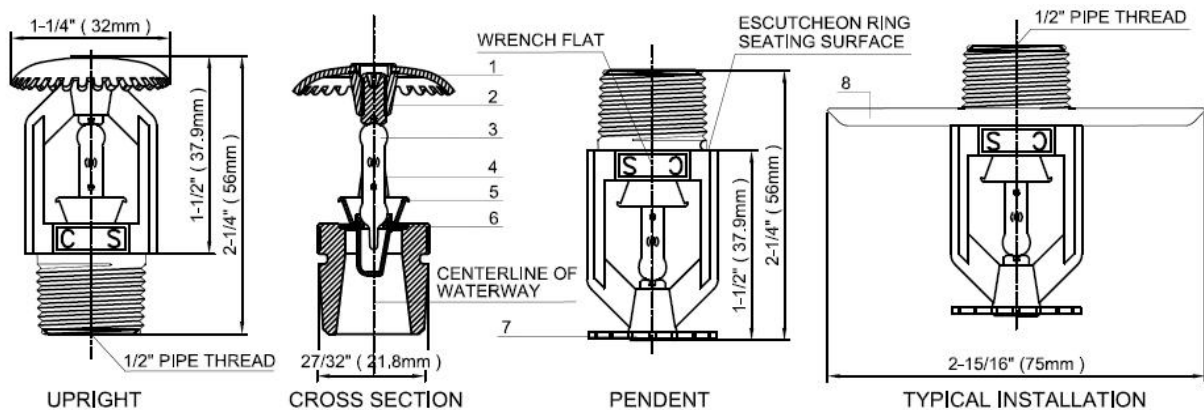
FIGURE A : MODEL NX023/NX024 UPRIGHT & MODEL NX025/NX026 PENDENT SPRINKLERS
